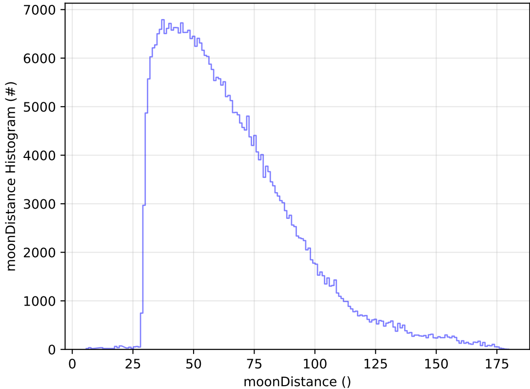
too_elab_2yr_r128_d2_griz_v3.4_10yrs WFD y band: moonDistance Histogram
