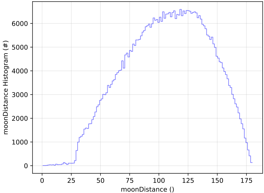
too_elab_2yr_r128_d2_griz_v3.4_10yrs WFD r band: moonDistance Histogram
