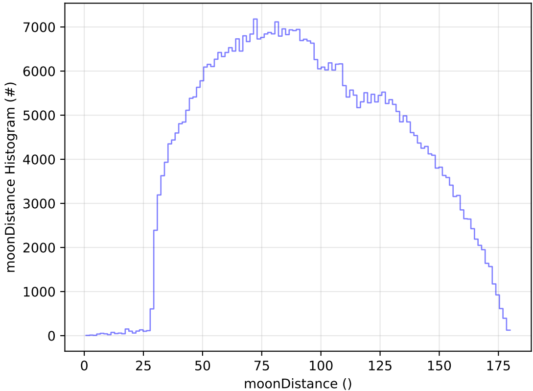
too_elab_2yr_r128_d2_griz_v3.4_10yrs WFD i band: moonDistance Histogram
