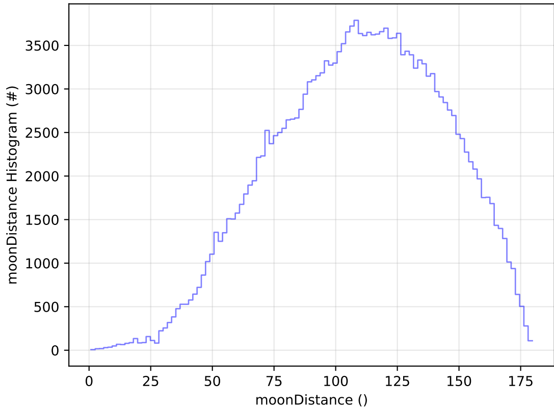
too_elab_2yr_r128_d2_griz_v3.4_10yrs WFD g band: moonDistance Histogram
