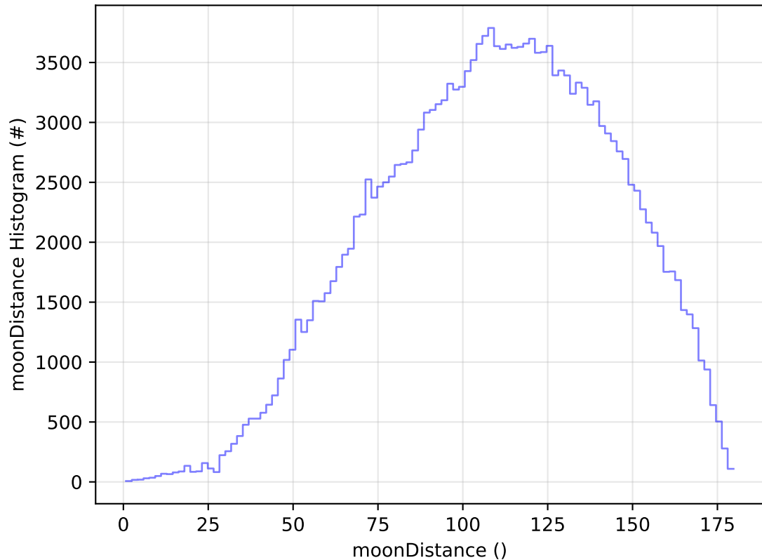
too_elab_2yr_r128_d2_griz_v3.4_10yrs All sky g band: moonDistance Histogram
