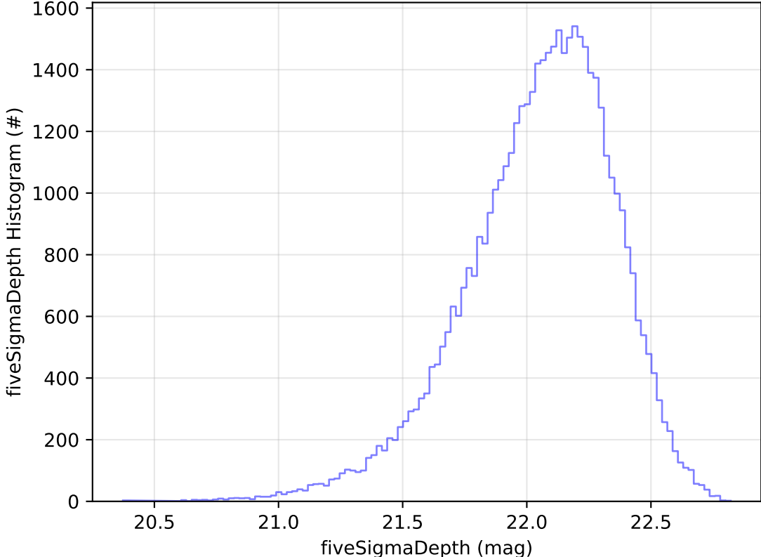
too_elab_2yr_r128_d2_griz_v3.4_10yrs Yr 1 y band: fiveSigmaDepth Histogram
