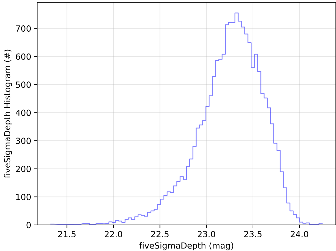
too_elab_2yr_r128_d2_griz_v3.4_10yrs Yr 1 u band: fiveSigmaDepth Histogram
