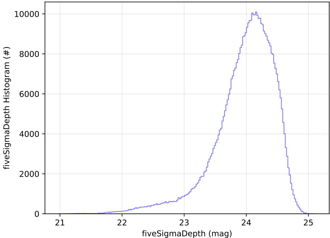
too_elab_2yr_r128_d2_griz_v3.4_10yrs WFD r band: fiveSigmaDepth Histogram
