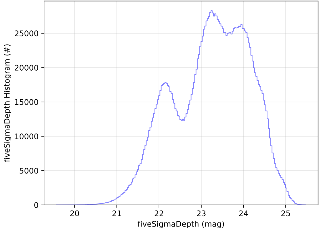
too_elab_2yr_r128_d2_griz_v3.4_10yrs WFD all bands: fiveSigmaDepth Histogram
