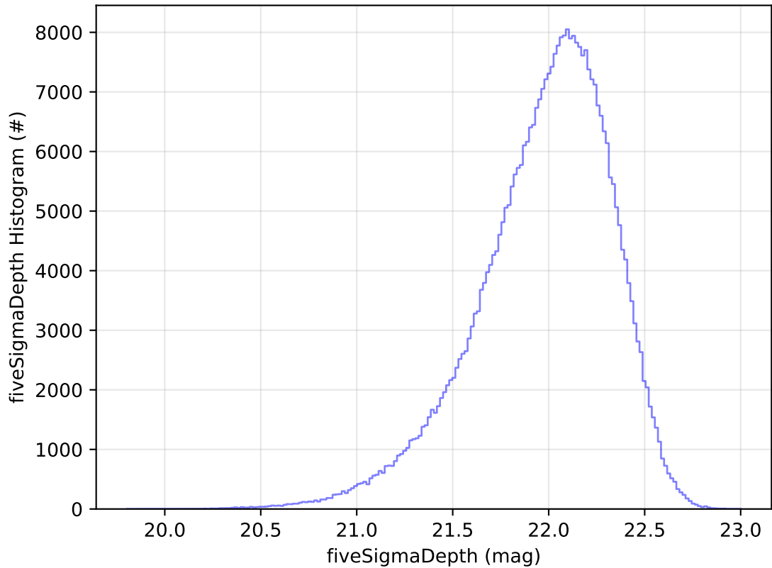
too_elab_2yr_r128_d2_griz_v3.4_10yrs All sky y band: fiveSigmaDepth Histogram
