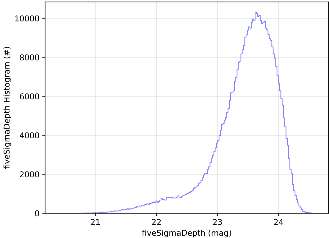
too_elab_2yr_r128_d2_griz_v3.4_10yrs All sky i band: fiveSigmaDepth Histogram
