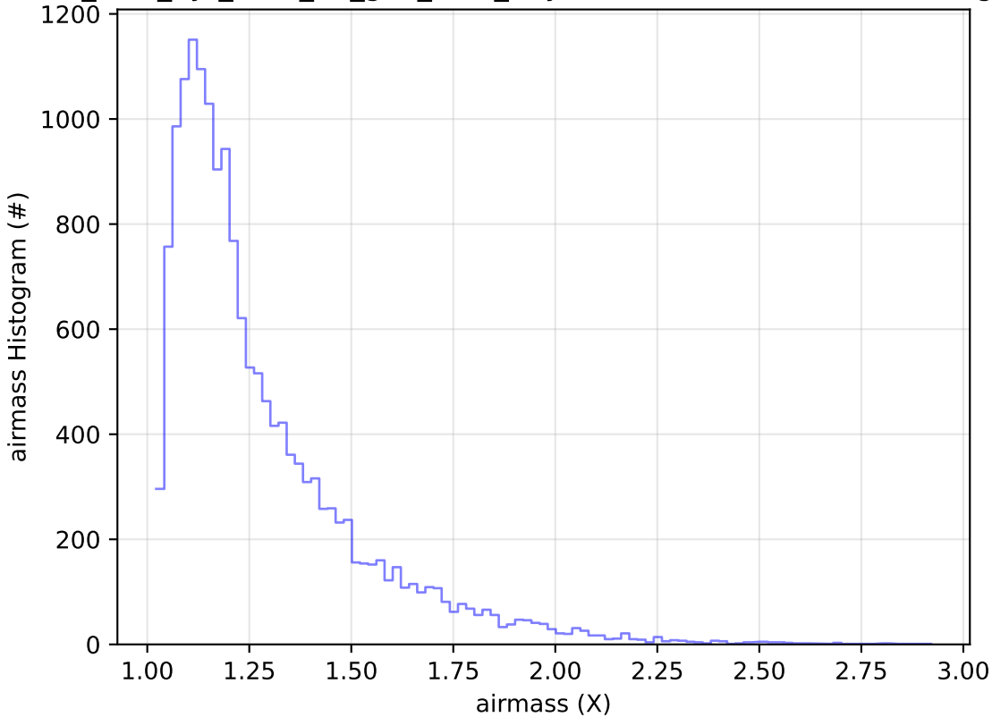
too_elab_2yr_r128_d2_griz_v3.4_10yrs Yr 1 u band: airmass Histogram
