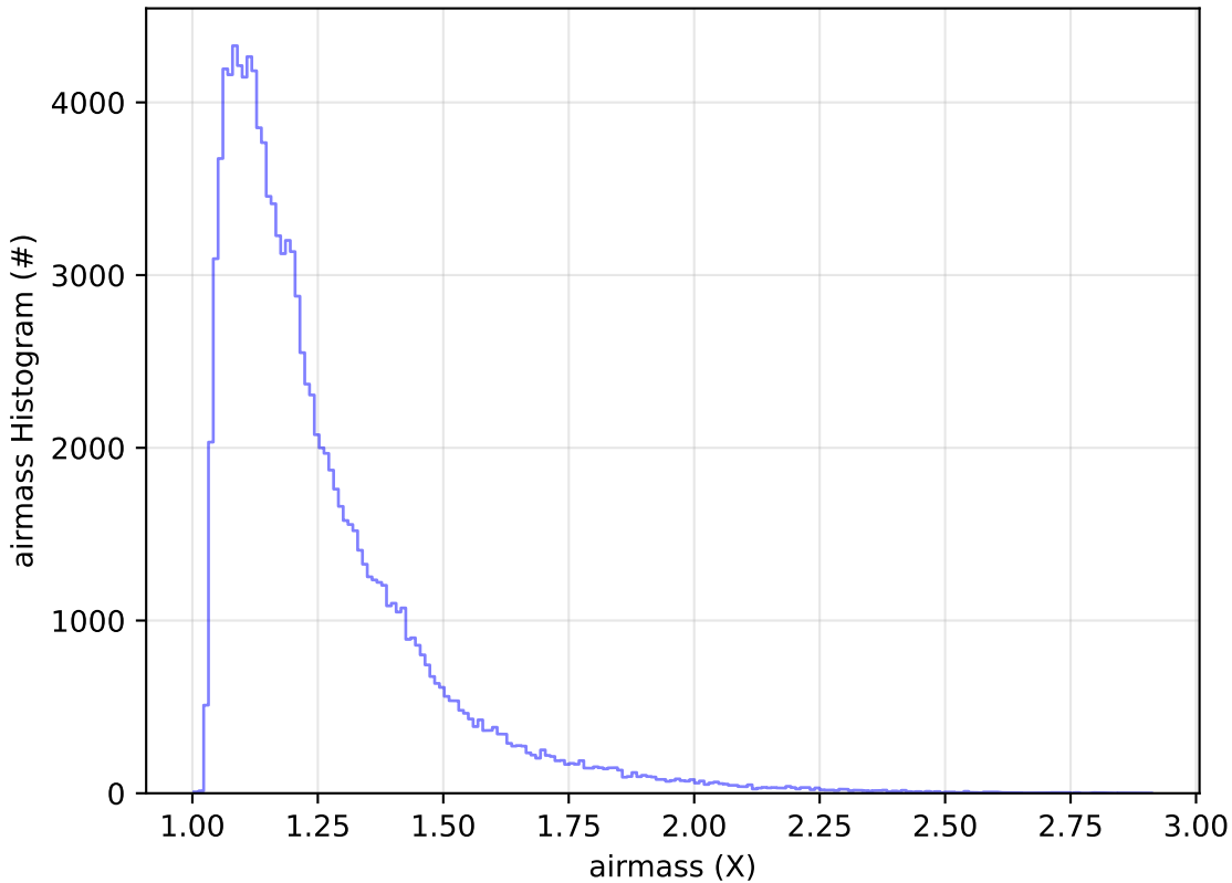
too_elab_2yr_r128_d2_griz_v3.4_10yrs WFD u band: airmass Histogram
