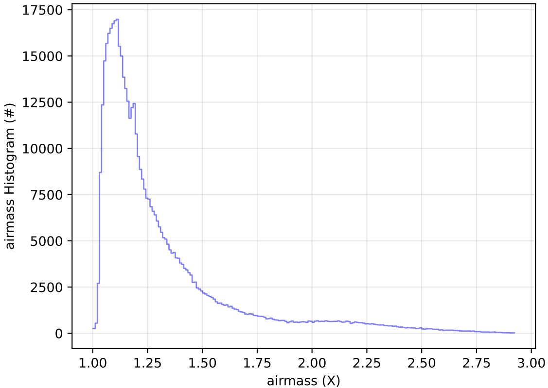
too_elab_2yr_r128_d2_griz_v3.4_10yrs WFD i band: airmass Histogram
