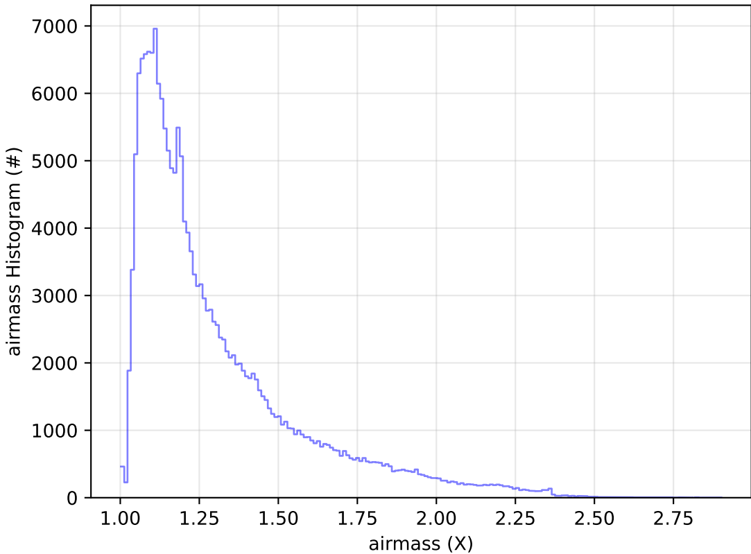
too_elab_2yr_r128_d2_griz_v3.4_10yrs WFD g band: airmass Histogram
