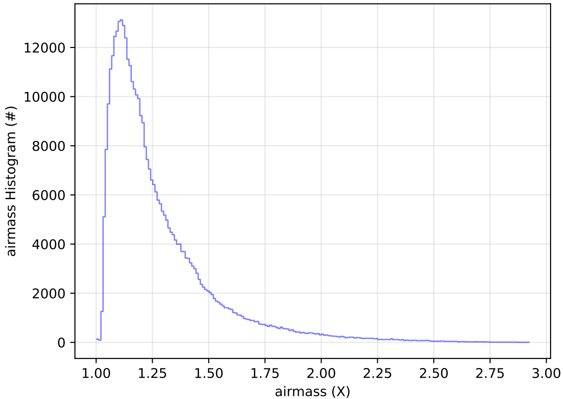
too_elab_2yr_r128_d2_griz_v3.4_10yrs All sky y band: airmass Histogram
