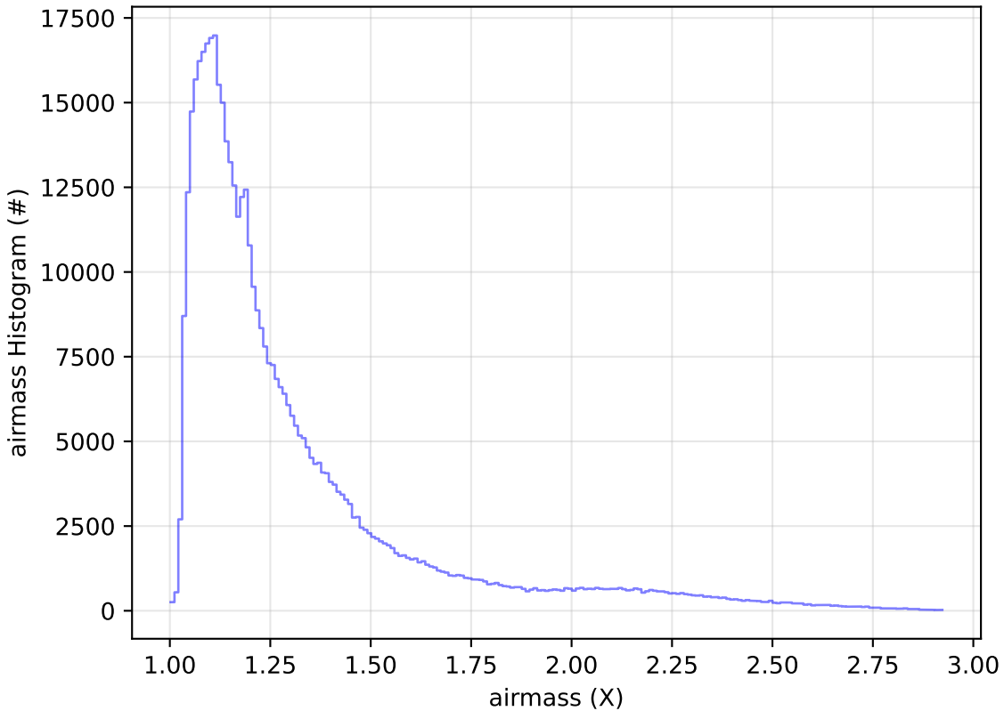
too_elab_2yr_r128_d2_griz_v3.4_10yrs All sky i band: airmass Histogram
