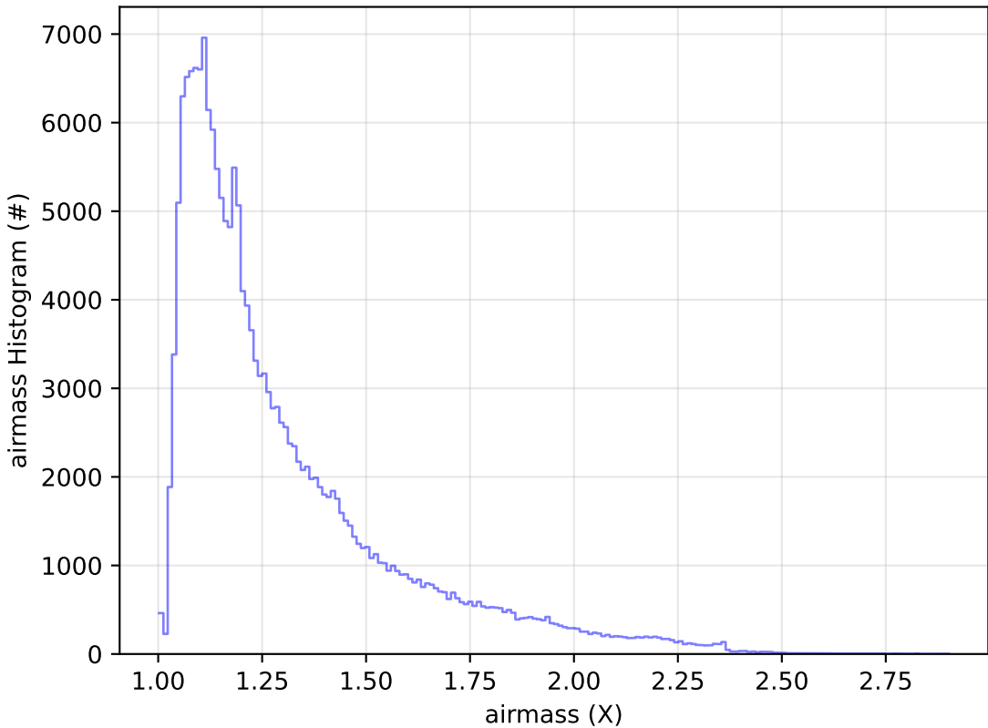
too_elab_2yr_r128_d2_griz_v3.4_10yrs All sky g band: airmass Histogram
