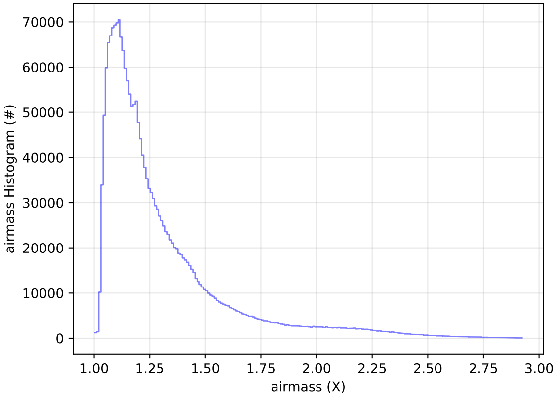
too_elab_2yr_r128_d2_griz_v3.4_10yrs All sky all bands: airmass Histogram
