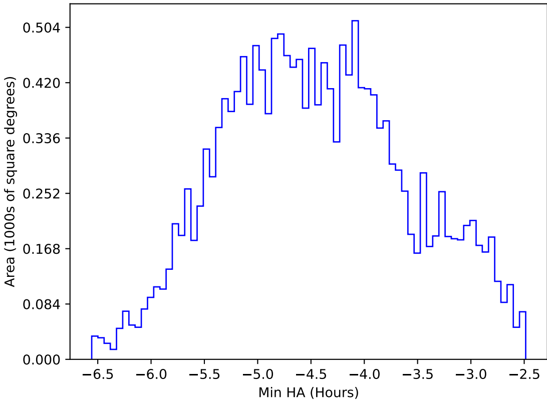
too_elab_2yr_r128_d2_griz_v3.4_10yrs WFD r band: Min HA
