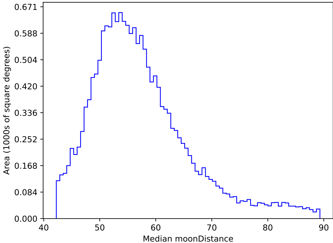
too_elab_2yr_r128_d2_griz_v3.4_10yrs WFD y band: Median moonDistance
