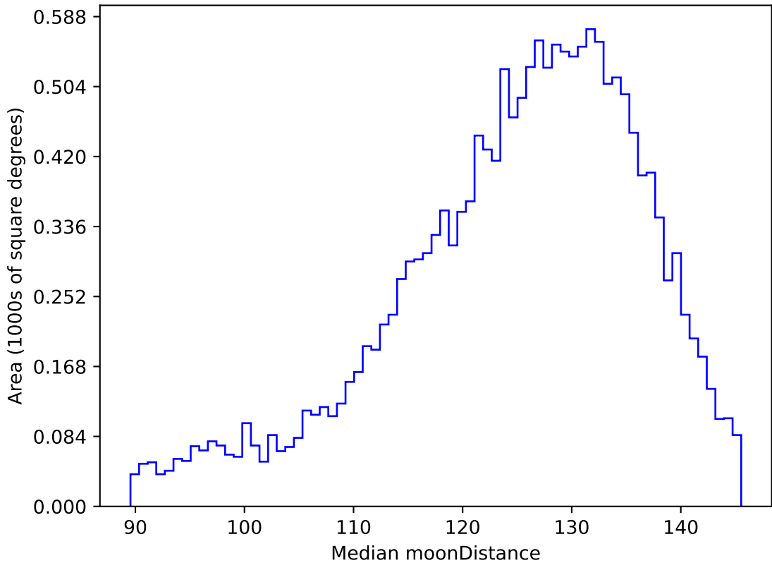
too_elab_2yr_r128_d2_griz_v3.4_10yrs WFD u band: Median moonDistance
