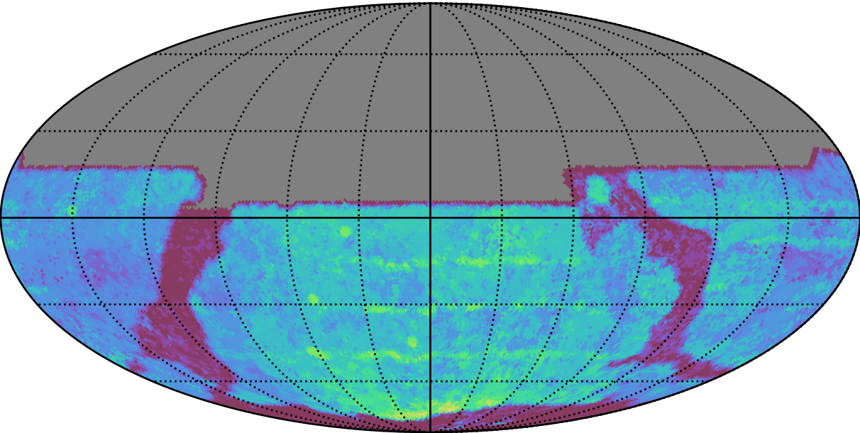
too_elab_2yr_r128_d2_griz_v3.4_10yrs All sky y band: Median Season Length
