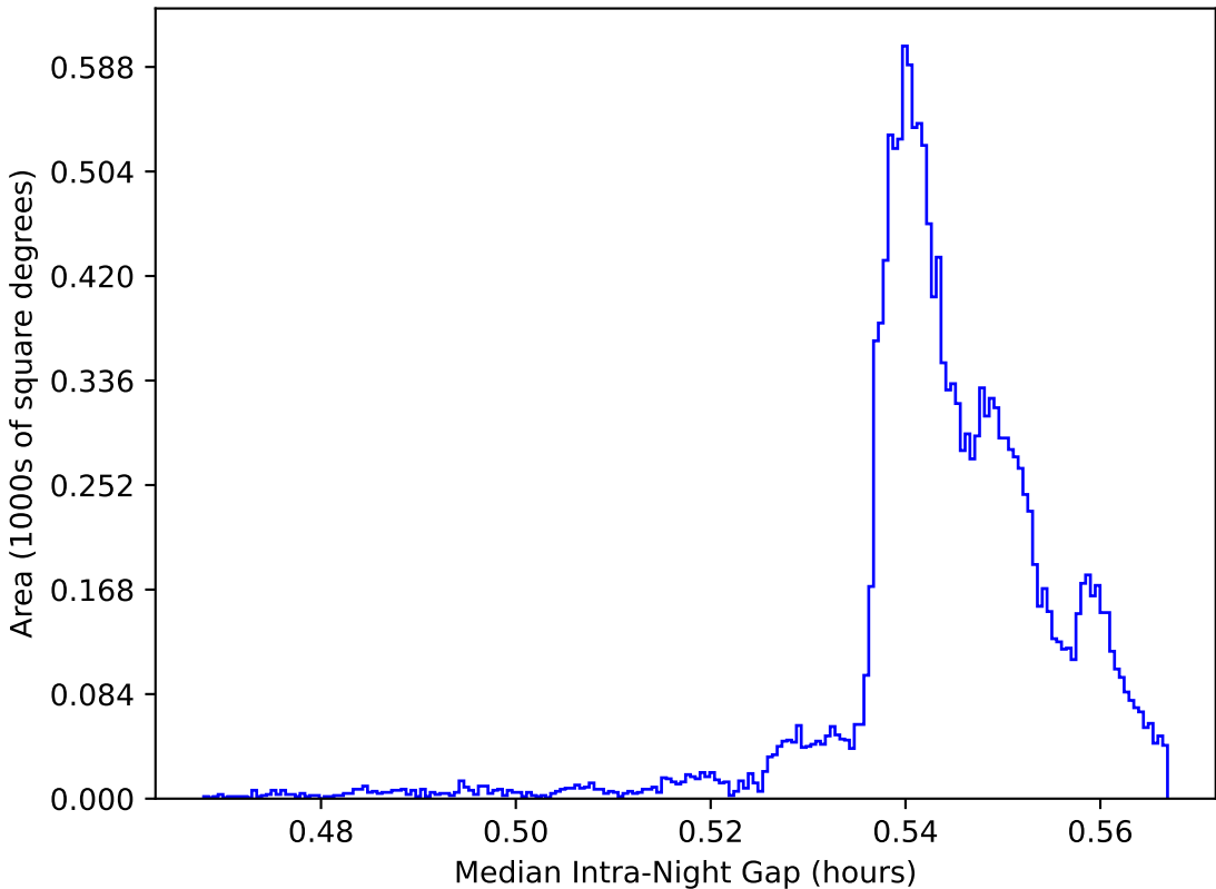
too_elab_2yr_r128_d2_griz_v3.4_10yrs WFD: Median Intra-Night Gap
