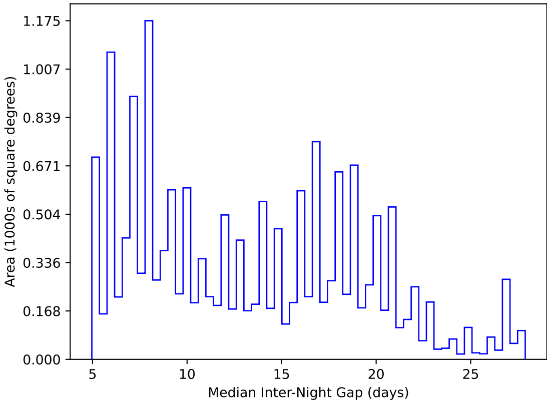
too_elab_2yr_r128_d2_griz_v3.4_10yrs WFD y band: Median Inter-Night Gap
