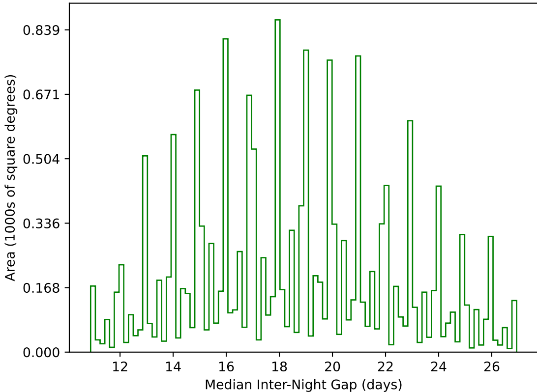
too_elab_2yr_r128_d2_griz_v3.4_10yrs WFD g band: Median Inter-Night Gap
