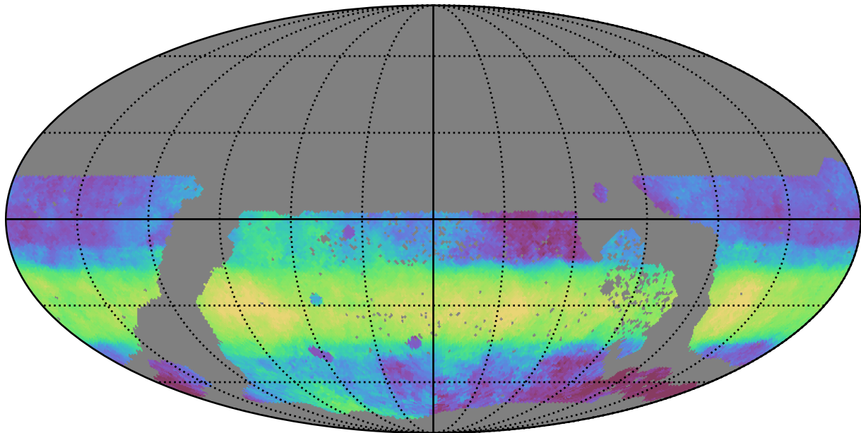
too_elab_2yr_r128_d2_griz_v3.4_10yrs WFD i band: Median HA
