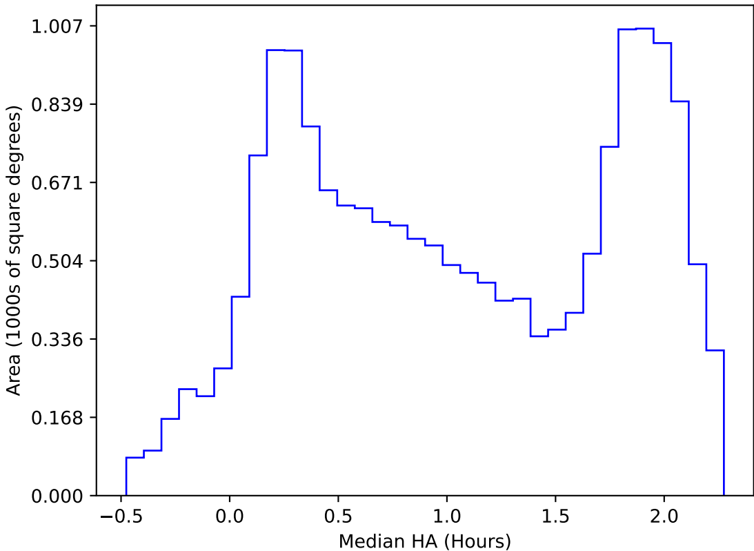
too_elab_2yr_r128_d2_griz_v3.4_10yrs WFD i band: Median HA
