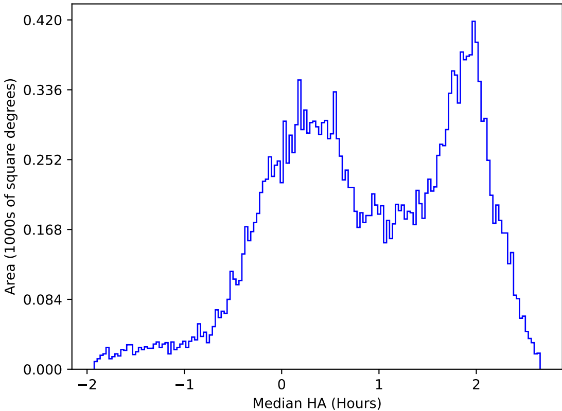
too_elab_2yr_r128_d2_griz_v3.4_10yrs All sky u band: Median HA
