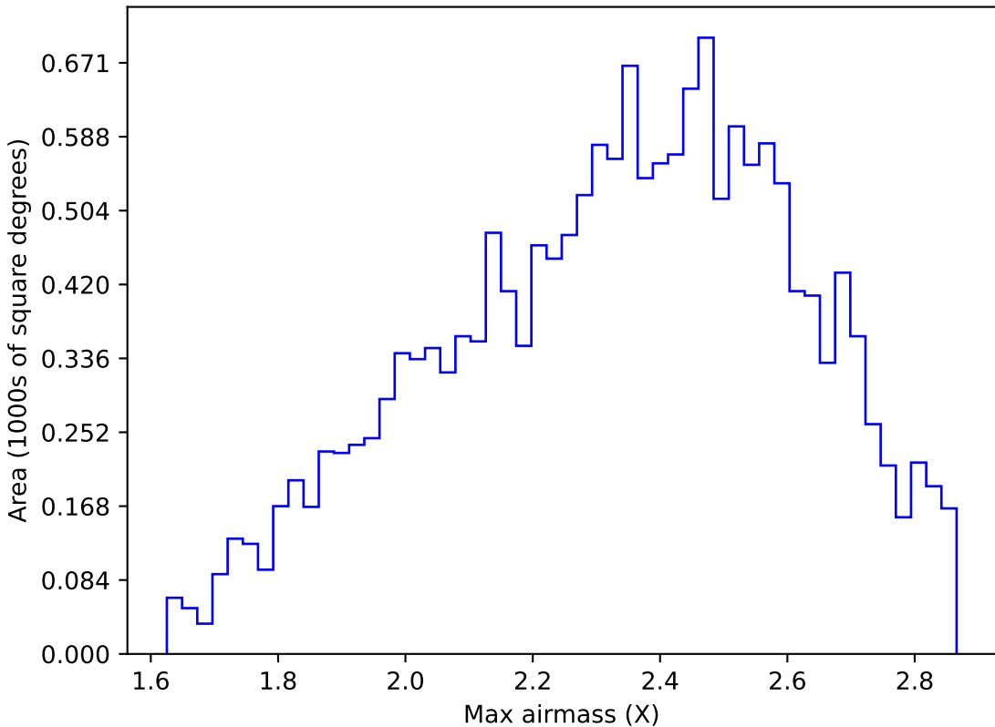
too_elab_2yr_r128_d2_griz_v3.4_10yrs WFD y band: Max airmass
