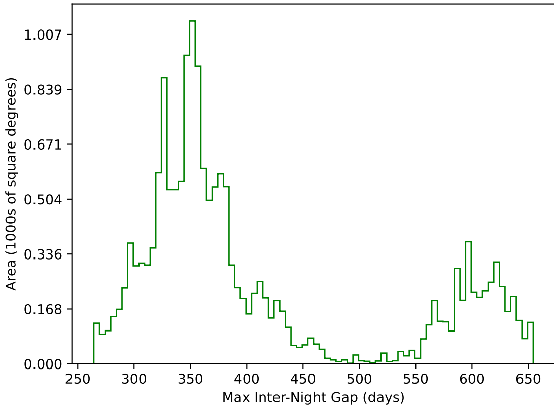
too_elab_2yr_r128_d2_griz_v3.4_10yrs WFD g band: Max Inter-Night Gap
