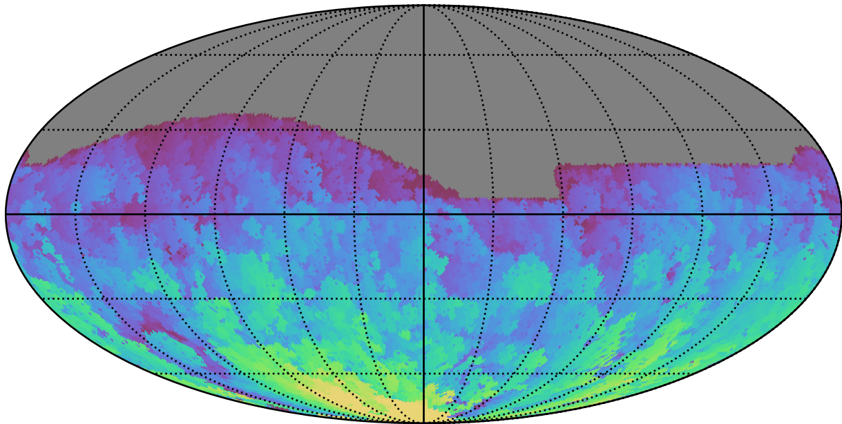
too_elab_2yr_r128_d2_griz_v3.4_10yrs All sky g band: Max HA
