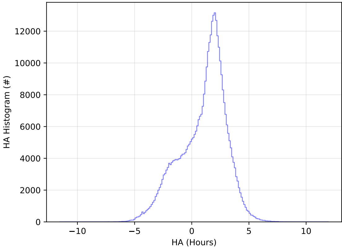
too_elab_2yr_r128_d2_griz_v3.4_10yrs WFD y band: HA Histogram
