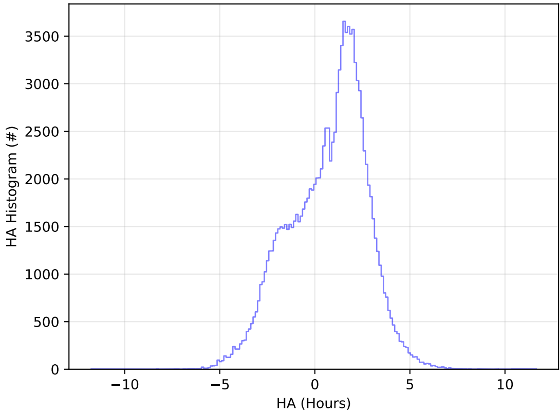
too_elab_2yr_r128_d2_griz_v3.4_10yrs WFD u band: HA Histogram
