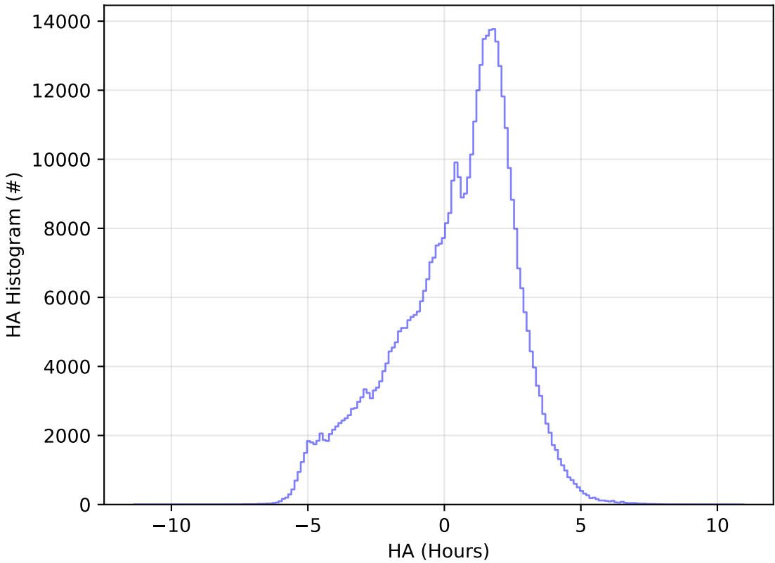
too_elab_2yr_r128_d2_griz_v3.4_10yrs WFD r band: HA Histogram
