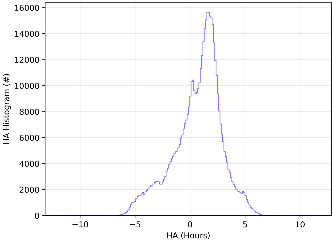
too_elab_2yr_r128_d2_griz_v3.4_10yrs WFD i band: HA Histogram
