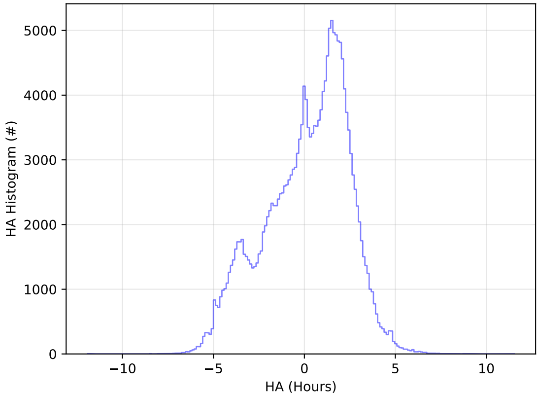
too_elab_2yr_r128_d2_griz_v3.4_10yrs WFD g band: HA Histogram
