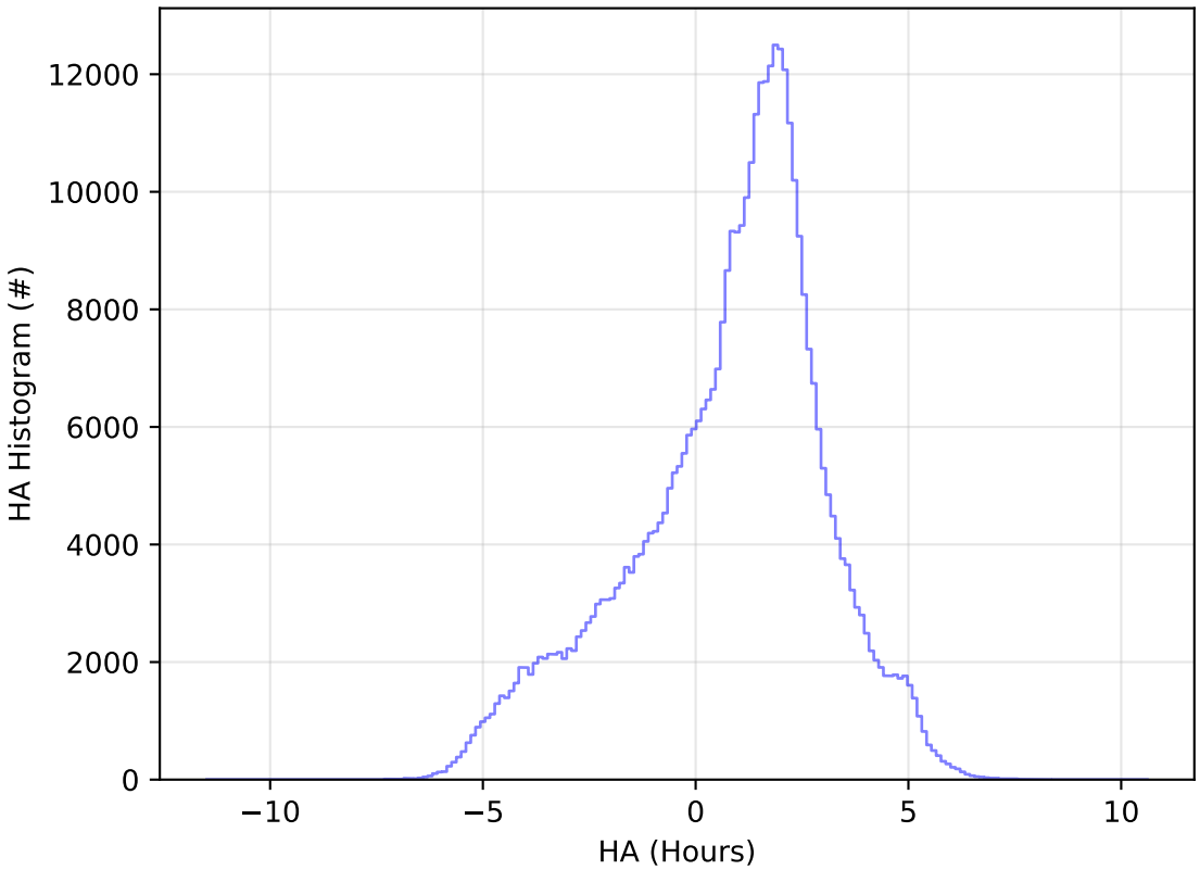
too_elab_2yr_r128_d2_griz_v3.4_10yrs All sky z band: HA Histogram
