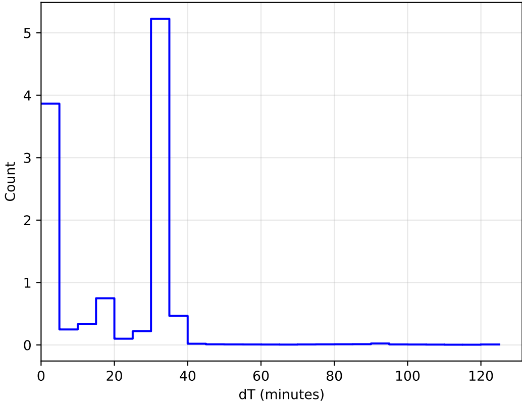
too_elab_2yr_r128_d2_griz_v3.4_10yrs WFD: DeltaT Histogram 1e6
