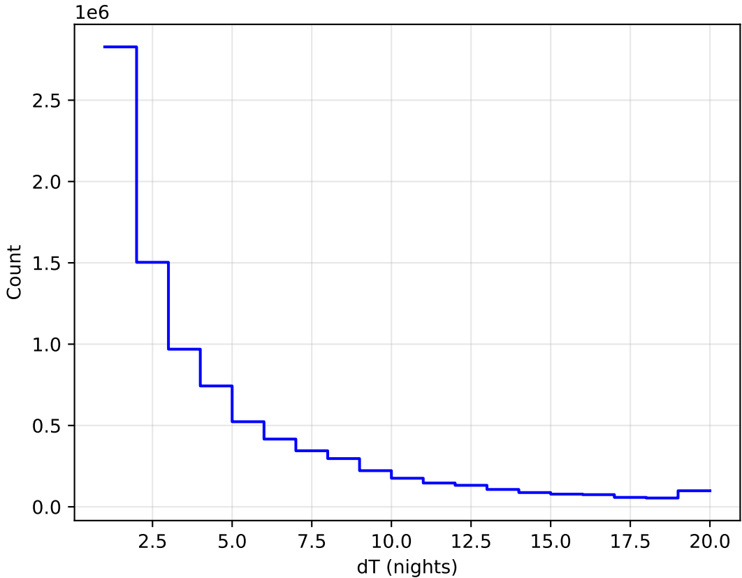
too_elab_2yr_r128_d2_griz_v3.4_10yrs All sky all bands: DeltaNight Histogram
