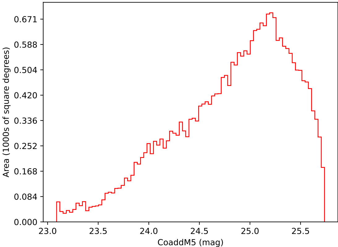
too_elab_2yr_r128_d2_griz_v3.4_10yrs Yr 3-4 i band: CoaddM5
