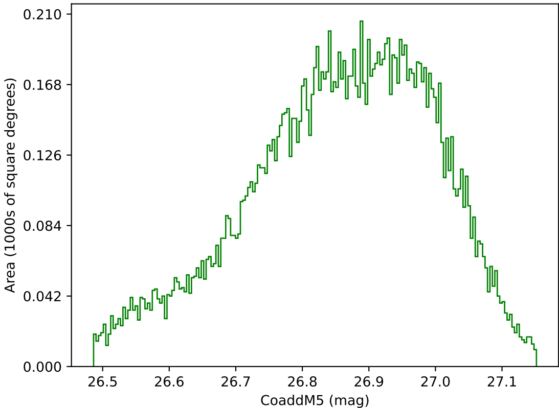
too_elab_2yr_r128_d2_griz_v3.4_10yrs WFD g band: CoaddM5
