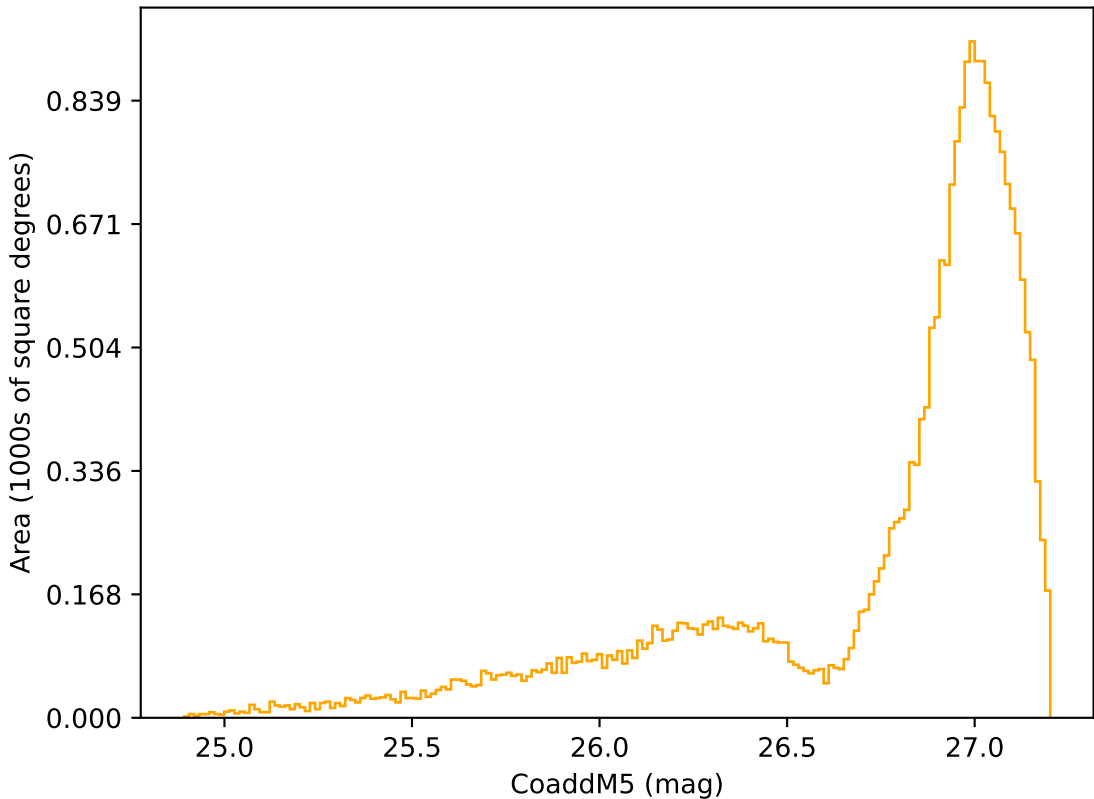
too_elab_2yr_r128_d2_griz_v3.4_10yrs All sky r band: CoaddM5
