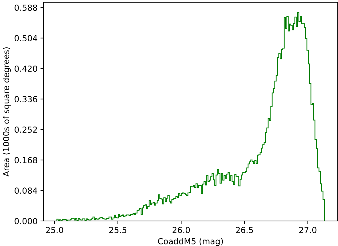
too_elab_2yr_r128_d2_griz_v3.4_10yrs All sky g band: CoaddM5
