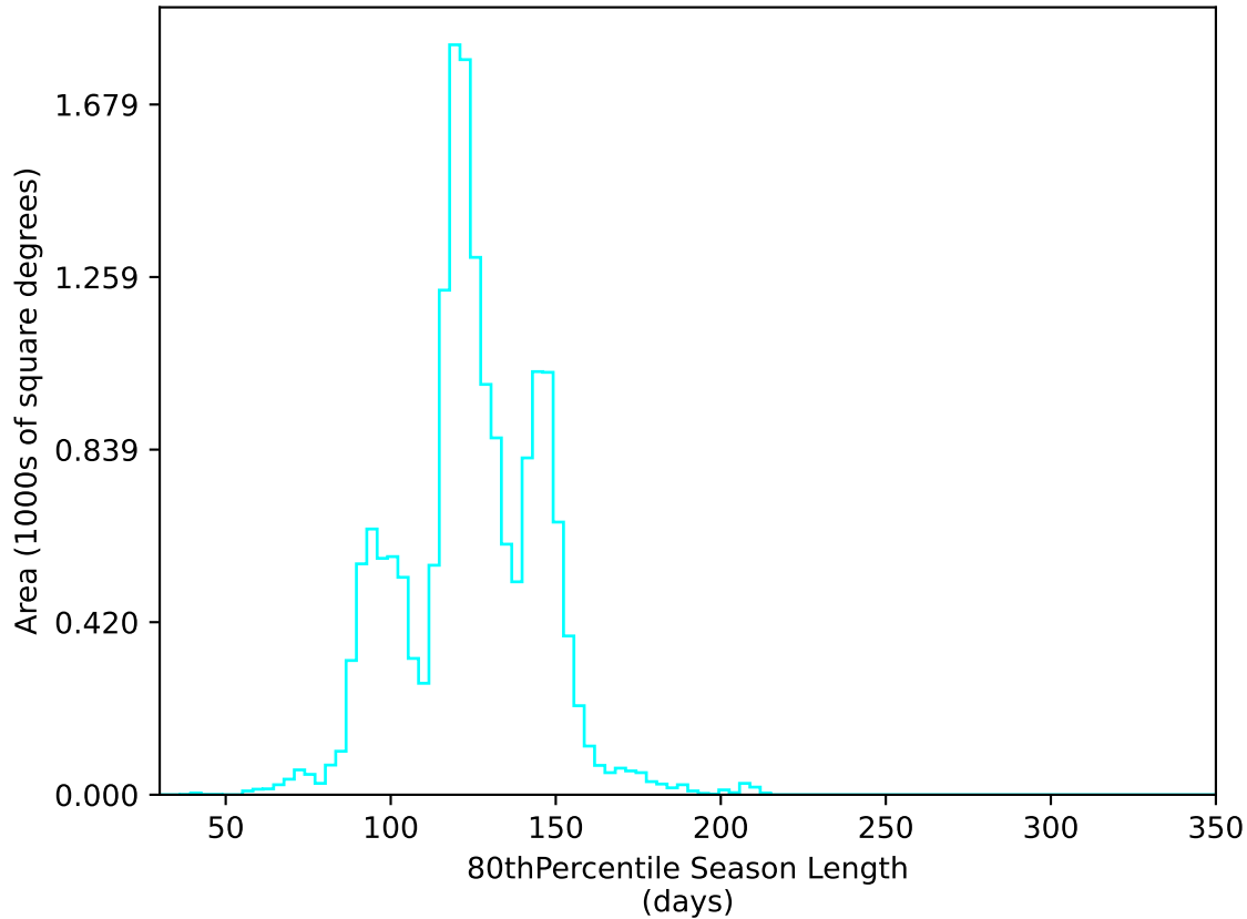
too_elab_2yr_r128_d2_griz_v3.4_10yrs WFD u band: 80thPercentile Season Length
