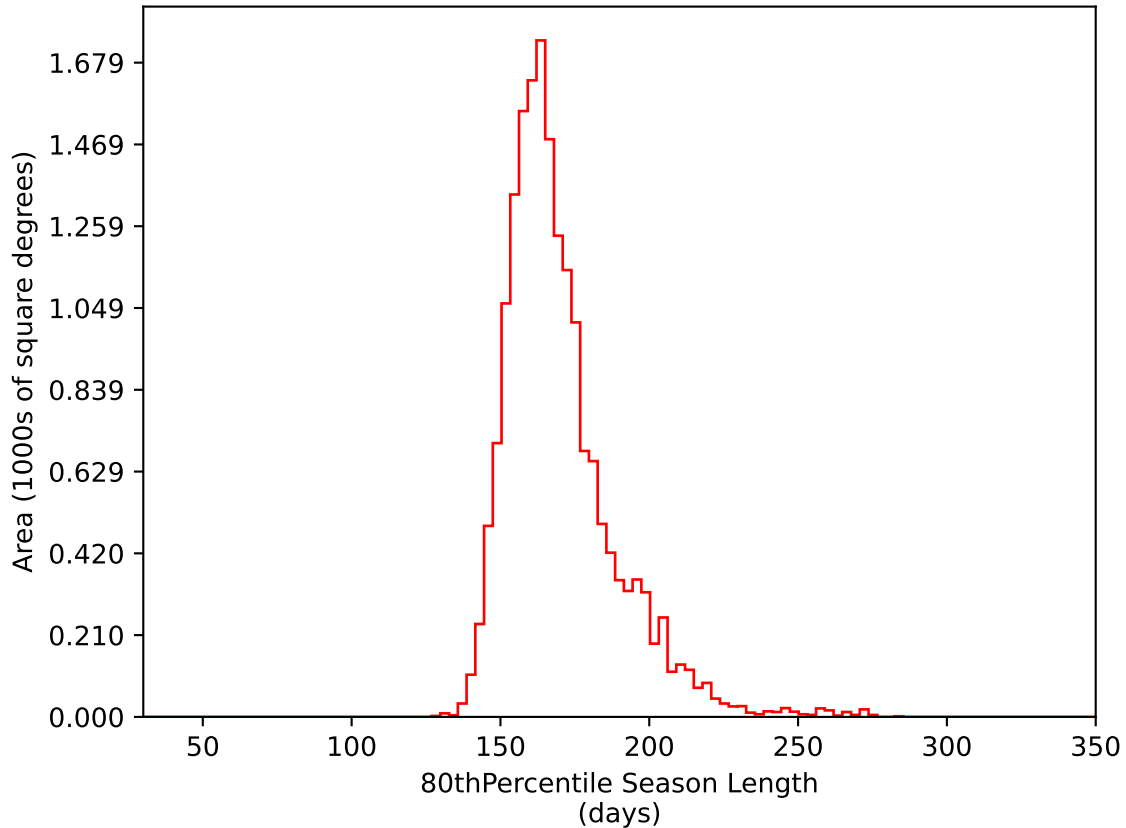
too_elab_2yr_r128_d2_griz_v3.4_10yrs WFD i band: 80thPercentile Season Length
