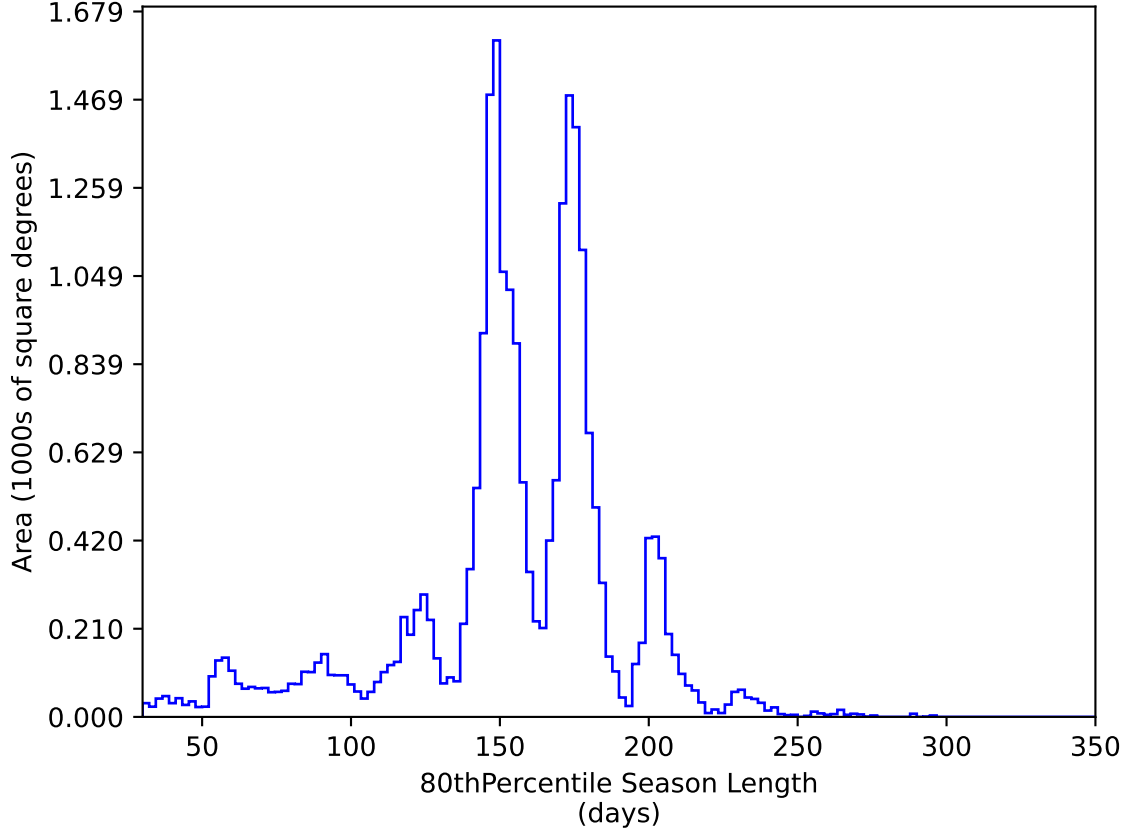
too_elab_2yr_r128_d2_griz_v3.4_10yrs All sky y band: 80thPercentile Season Length
