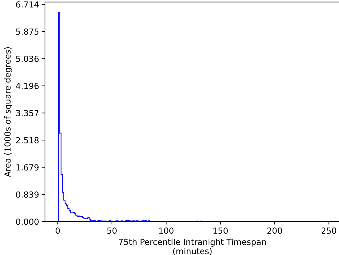
too_elab_2yr_r128_d2_griz_v3.4_10yrs WFD u band: 75th Percentile Intranight Timespan
