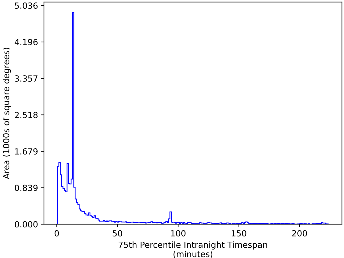
too_elab_2yr_r128_d2_griz_v3.4_10yrs All sky z band: 75th Percentile Intranight Timespan
