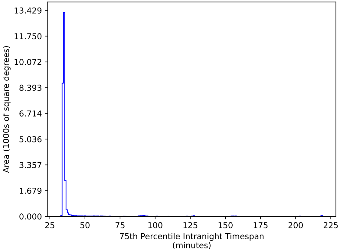
too_elab_2yr_r128_d2_griz_v3.4_10yrs All sky ri bands: 75th Percentile Intranight Timespan
